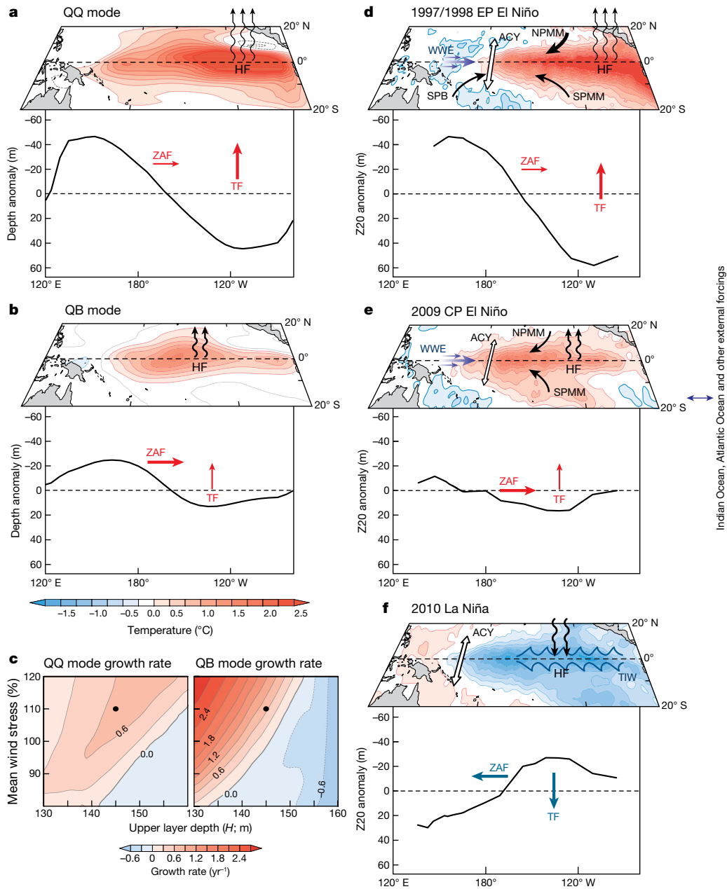
Fig. 5 | Mechanisms of ENSO complexity. a, b , Leading two eigenmodes of tropical Pacific SSTA and equatorial thermocline depth anomalies (averaged between 5° S–5° N) with periods of about 4 yr (QQ, quasi-quadrennial) and about 2 yr (QB, quasi-biennial), calculated from an intermediate ENSO model 46 . The differences in zonal location of the centre in SSTAs and thermocline anomalies are largely due to the different roles of the zonal advective feedback (ZAF) and thermocline feedback (TF). c , Growth rates of the two eigenmodes as a function of the mean thermocline depth, H , and the mean strength of equatorial trade winds relative to climatological conditions. Black dots mark the mean state for the modes displayed in a and b . d–f , Patterns of SSTAs 26 and equatorial Tropical Atmosphere Ocean (TAO)/ Triangle Trans-Ocean Buoy Network
