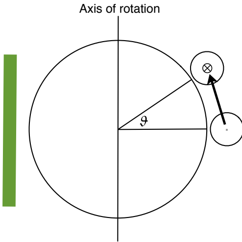
Figure 11.5 If a ring of air at the equator moves polewards it moves closer to the axis of rotation. If the parcels in the ring conserve their angular momentum their zonal velocity must increase; thus, if m = (\bar{u} + \Omega a \cos \vartheta)a \cos \vartheta is preserved and \bar{u} = 0 at \vartheta = 0 we recover (11.7).
