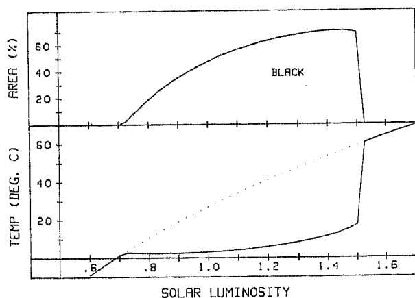
Fig. 2. Steady state response for conditions as in Fig. 1d, but with a cloud of albedo 0.8 assumed to obscure the black daisies.
