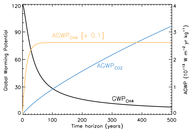
Figure 8.29 | Development of AGWP- \text{CO}_2 , AGWP- \text{CH}_4 and GWP- \text{CH}_4 with time horizon. The yellow and blue curves show how the AGWPs changes with increasing time horizon. Because of the integrative nature the AGWP for \text{CH}_4 (yellow curve) reaches a constant level after about five decades. The AGWP for \text{CO}_2 continues to increase for centuries. Thus the ratio which is the GWP (black curve) falls with increasing time horizon.
