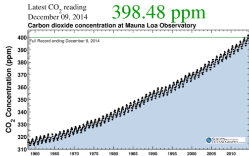
The Keeling Curve, December 2014, Scripps Institution of Oceanography, UC San Diego
