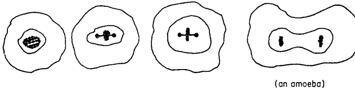
FIG. 2. Mitotic figures of some representative eukaryotes. These figures were adapted from the illustrations which may be found in the references cited. The names of the organisms given are generic. The name in parenthesis indicates the larger group in which the organism can be found in Fig. 1, the phylogenetic tree. A common description is given for some of the more obscure genera. The Roman numeral groups correspond to branches on the phylogenetic tree as discussed in sections 2.5.1 to 2.5.6 of the text. The organisms in groups I, III and V are thought to be premitotic. In groups II, IV and VI the subgroupings A and B refer to "premitotic" and "eumitotic", respectively. [The lower case letters (a), (b) . . . are simply included for reference.]
