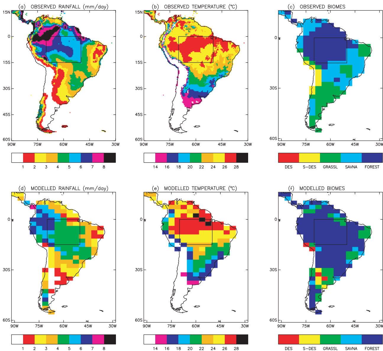
Fig. 2. Rainfall, screen-level air temperature and biome distributions over South America from observational datasets ( a, b, c ) and the model simulation of the pre-industrial state ( d, e, f ). Climate observations are from New et al. (1999) and the biome distribution is derived from Loveland et al. (2000)
