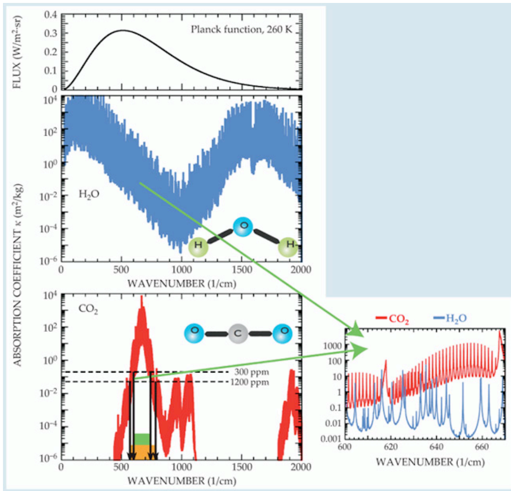
FIGURE 2. Absorption coefficients for water vapor and carbon dioxide as a function of wavenumber are synthesized here from spectral line data in the HITRAN database. The upper panel gives the Planck function B(\nu, T) for a 260-K surface, which indicates the spectral regions that are important for planetary energy balance. The wavenumber, defined as the reciprocal of the wavelength, is proportional to frequency. If a layer of atmosphere contains M kilograms of absorber for each square meter at the base of the layer, then light is attenuated by a factor \exp(-\kappa M) when crossing the layer, where \kappa is the absorption coefficient. The horizontal dashed lines on the CO 2 plot give the value of absorption coefficient above which the atmosphere becomes very strongly absorbing for CO 2 concentrations of 300 ppm and 1200 ppm; the green rectangle shows the portion of the spectrum in which the atmosphere is optically thick for the lower concentration, and the orange rectangle indicates how the optically thick region expands as the concentration increases. The inset shows fine structure due to rotational levels.
