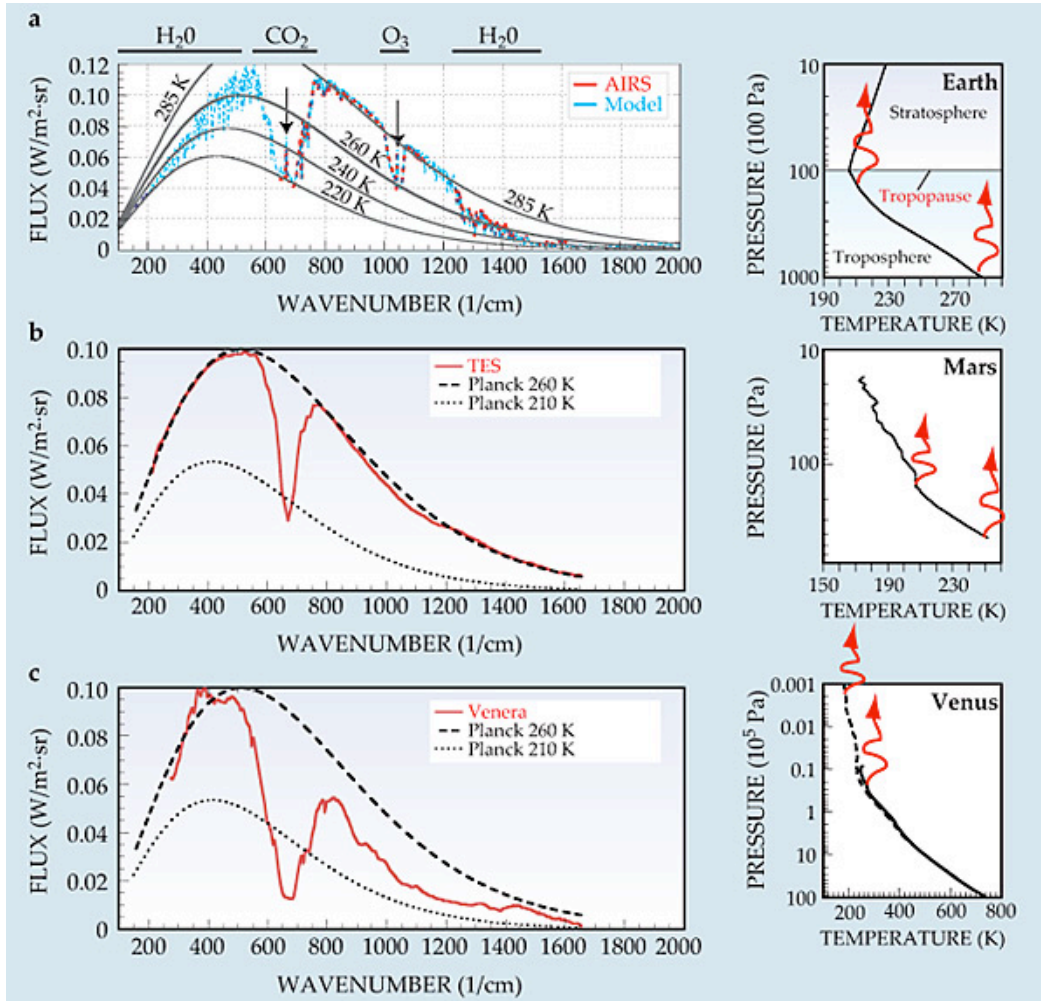
FIGURE 3. Satellite measurements of emission spectra are not limited to Earth. (a) The left panel compares a computed global-mean, annual-mean emission spectrum for Earth (blue) with observations from the satellite-borne AIRS instrument (red); both are superimposed over a series of Planck distributions. Two arrows point to absorption spikes discussed in the text. The temperature profile to the right, also an annual and global average, is based on in situ measurements. (b) The panel to the left shows a summer-afternoon emission spectrum for Mars observed by the TES instrument on the Mars Global Surveyor. Its accompanying temperature profile was obtained from radio-occultation measurements corresponding to similar conditions. (c) The panels here show a Venusian equatorial night thermal spectrum as measured by the Venera 15 orbiter[14] together with a typical temperature profile for the planet. The upper portion (dashed curve) of the temperature sounding is based on radio-occultation observations from the Magellan mission; the lower portion (solid curve) was observed by a Pioneer Venus descender probe. For all three planets, squiggly arrows on the temperature profiles indicate the range of altitudes from which IR escapes to space.
