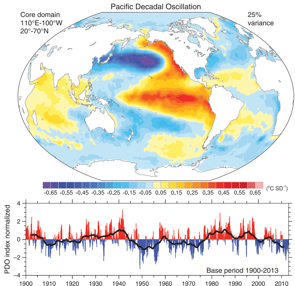
Figure 8. The Pacific Decadal Oscillation based on an EOF analysis of SST anomalies with the global mean removed from 1900 to May 2013 in the 20°N–70°N and 110°E–100°W region of the North Pacific, which explains 25% of the variance. The principal component time series, given below in normalized units, is regressed on global SSTs to give the map above. The black curve is a 61 month running average.
