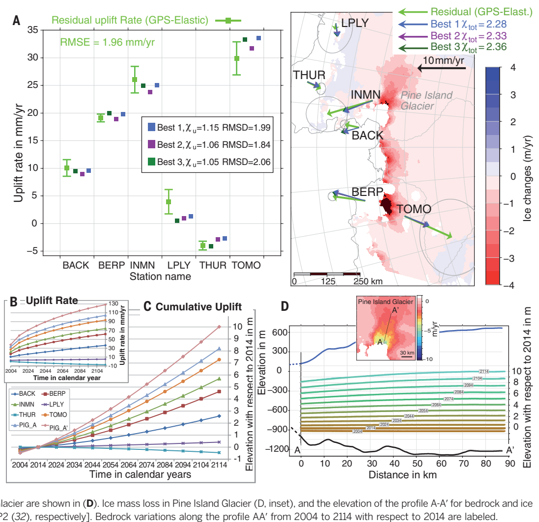
Fig. 3. Vertical and horizontal bedrock motion predictions. (A) The vertical (left) and horizontal (right) observed GPS minus elastic modeled residual velocities (green dot in left plot, green arrows in right plot) as in column 5 of table S2. Vertical and horizontal velocity predictions from three viscosity models providing good fit ( R^2 = 0.96 ) are shown by the blue (Best 1), purple (Best 2), and dark green (Best 3) symbols. These models are our three best-fitting models (the total \chi is reported in the legend of the right plot). In the text we indicate Best 2 as our preferred model because it has the lowest RMSD for the uplift rates. The error bars (left) are the weighted errors (error bar = SD/weight). The ellipses in (A) (right) represent uncertainties ( \pm 1 SD) for the associated residual horizontal velocity vectors. The weights are 1 except for LPLY and the horizontal for TOMO. Assuming that the current rate of ice thinning will be constant in the ASE throughout the next century, the evolution of uplift rates (B) and uplift (C) at the six GPS sites and points A and A' of the profile along Pine Island Glacier are shown in (D). Ice mass loss in Pine Island Glacier (D, inset), and the elevation of the profile A-A' for bedrock and ice [black and blue line from BEDMAP2 (32), respectively]. Bedrock variations along the profile AA' from 2004 to 2114 with respect to 2014 are labeled.
