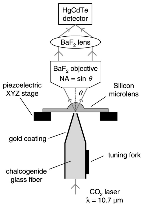
FIG. 1. Experimental setup used for refraction contrast imaging with a scanned Si microlens showing the stationary chalcogenide glass fiber source and BaF 2 objective with maximum collection angle \theta=46.7^\circ (NA=0.45).
