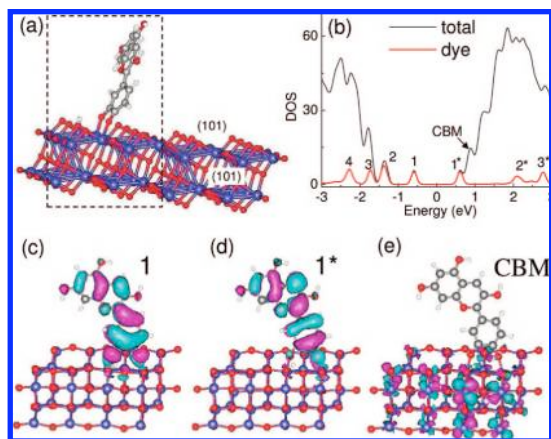
Figure 3. (a) Structure of the dye-sensitized \text{TiO}_2 [1\bar{1}1] -wire with all facets being (101). Dashed lines mark the unit cell in the calculation. (b) Total (thin black line) and projected (thick red line) density of states for this system. The corresponding wave functions for the (c) HOMO, (d) LUMO, and (e) LUMO + 1 states at the \Gamma k-point.
