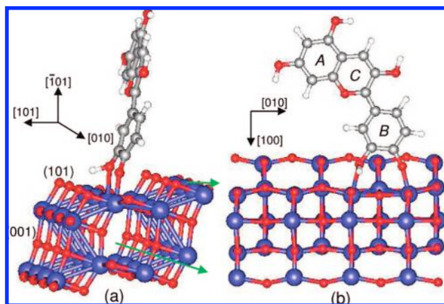
Figure 1. Unit cell for a prototypical TiO 2 nanowire sensitized by the cyanidin dye: (a) side view; (b) top view. Ti, O, C, and H atoms are represented by blue, red, gray, and white spheres, respectively. Green arrows indicate two possible nanowire axis directions.
