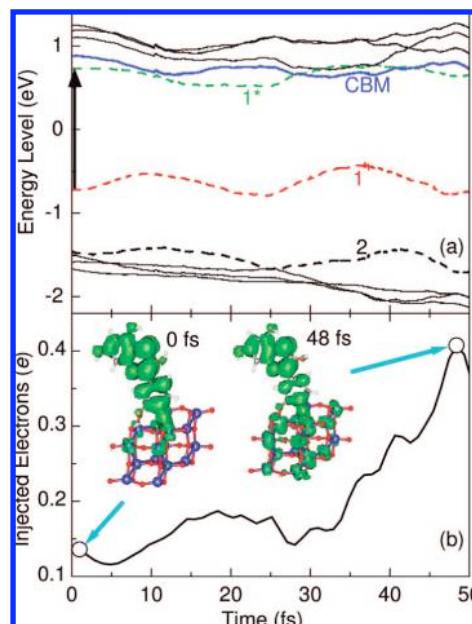
Figure 5. (a) Evolution of electronic state energy levels after excitation of cyanidin from its HOMO (state 1) to the LUMO (state 1*). Energy levels contributed by the dye are shown in dotted lines. (b) Fraction of electrons injected to the TiO 2 nanowire as a function of time after excitation. The insets show the charge density of the excited electron at t = 0 and 48 fs at the contour level of 0.004 e/\text{Å}^3 .
