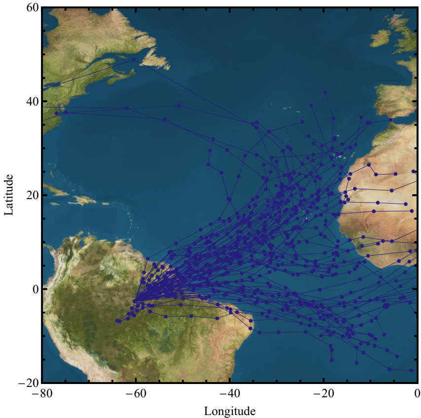
10-day backtrajectories at 2000 m every 12 h from 7 Feb to 14 Mar
