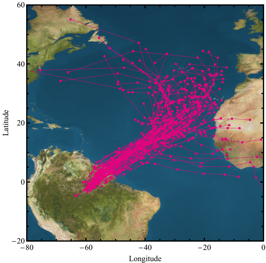
10-day backtrajectories at 500 m every 12 h from 7 Feb to 14 Mar
