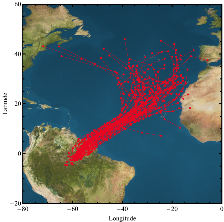
10-day backtrajectories at 200 m every 12 h from 7 Feb to 14 Mar
