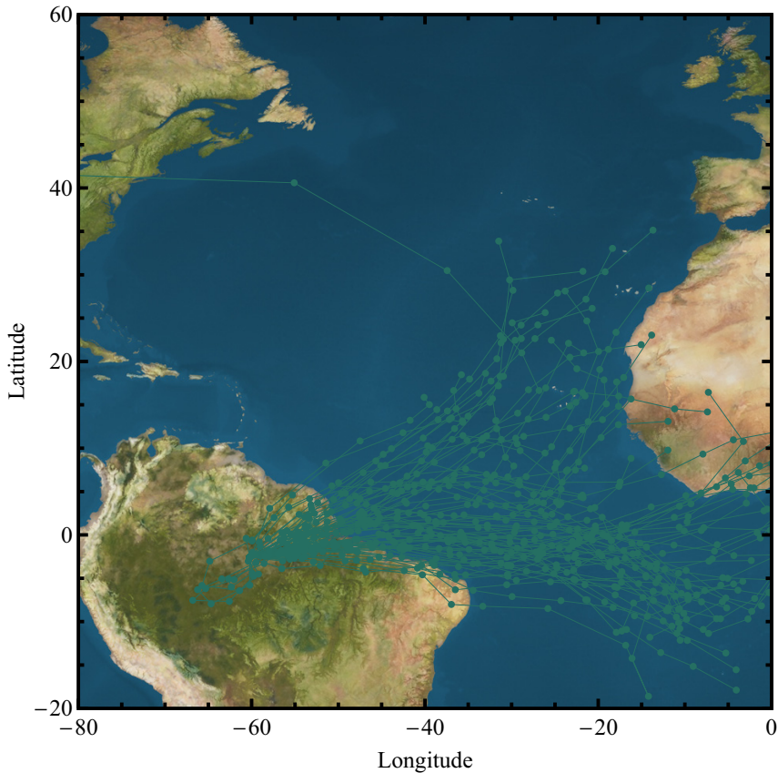
10-day backtrajectories at 4000 m every 12 h from 7 Feb to 14 Mar
