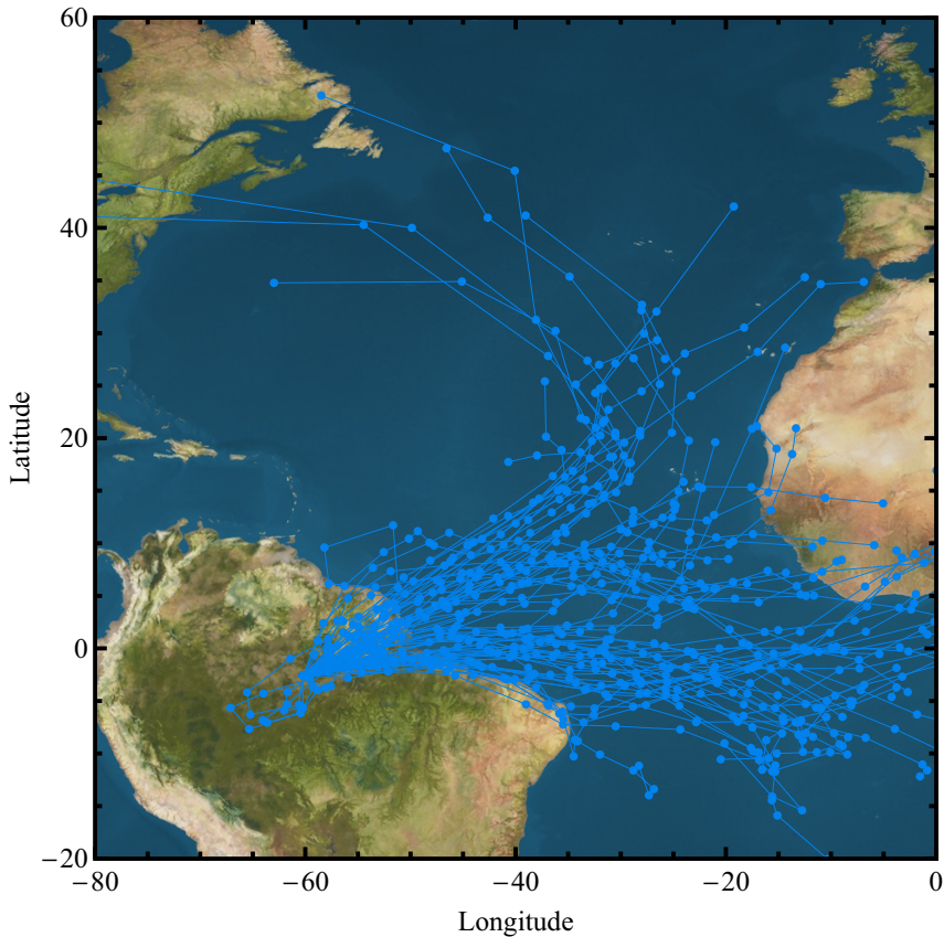
10-day backtrajectories at 3000 m every 12 h from 7 Feb to 14 Mar
