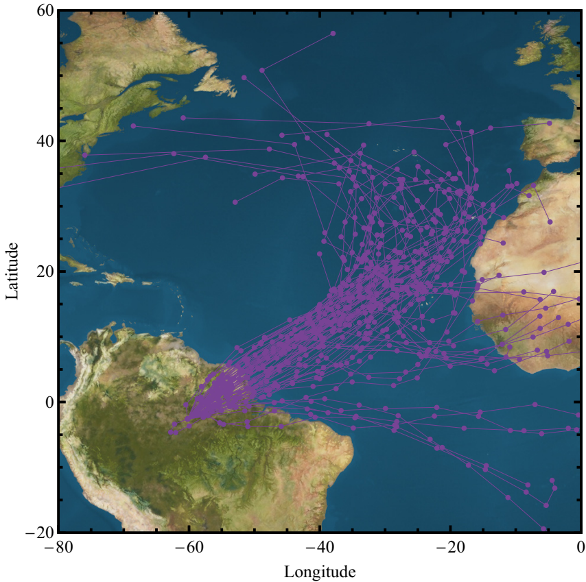
10-day backtrajectories at 1000 m every 12 h from 7 Feb to 14 Mar
