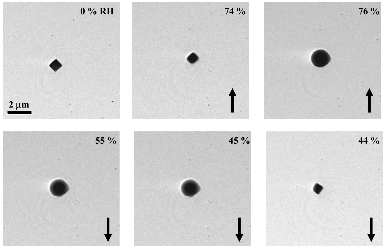
Figure 4. Images of a laboratory-generated NaCl particle ( \sim 1 \mu\text{m} ) as RH is increased from 0 to 76% and decreased from 76 to 44% (denoted by down arrows).
