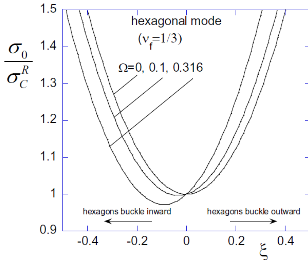
Fig. 11 Effect of spherical curvature on the relation between the applied stress and the buckling amplitude for the hexagonal mode. The centers of the hexagon prefer to buckle towards the concave (inward) side of the curved film.
