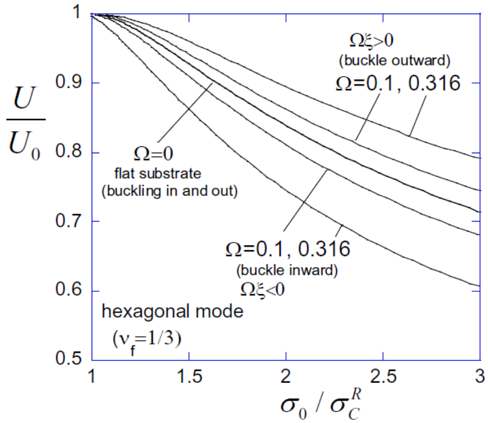
Fig. 12 Effect of curvature on the energy in the buckled states of the hexagonal mode.
