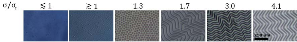
Fig. 3 Progression of modes observed experimentally for the UVO-treated PDMS system with increasing overstress as described in the text. The UVO treatment times from left to right are 10, 15, 20, 30, 45, and 60 minutes.
