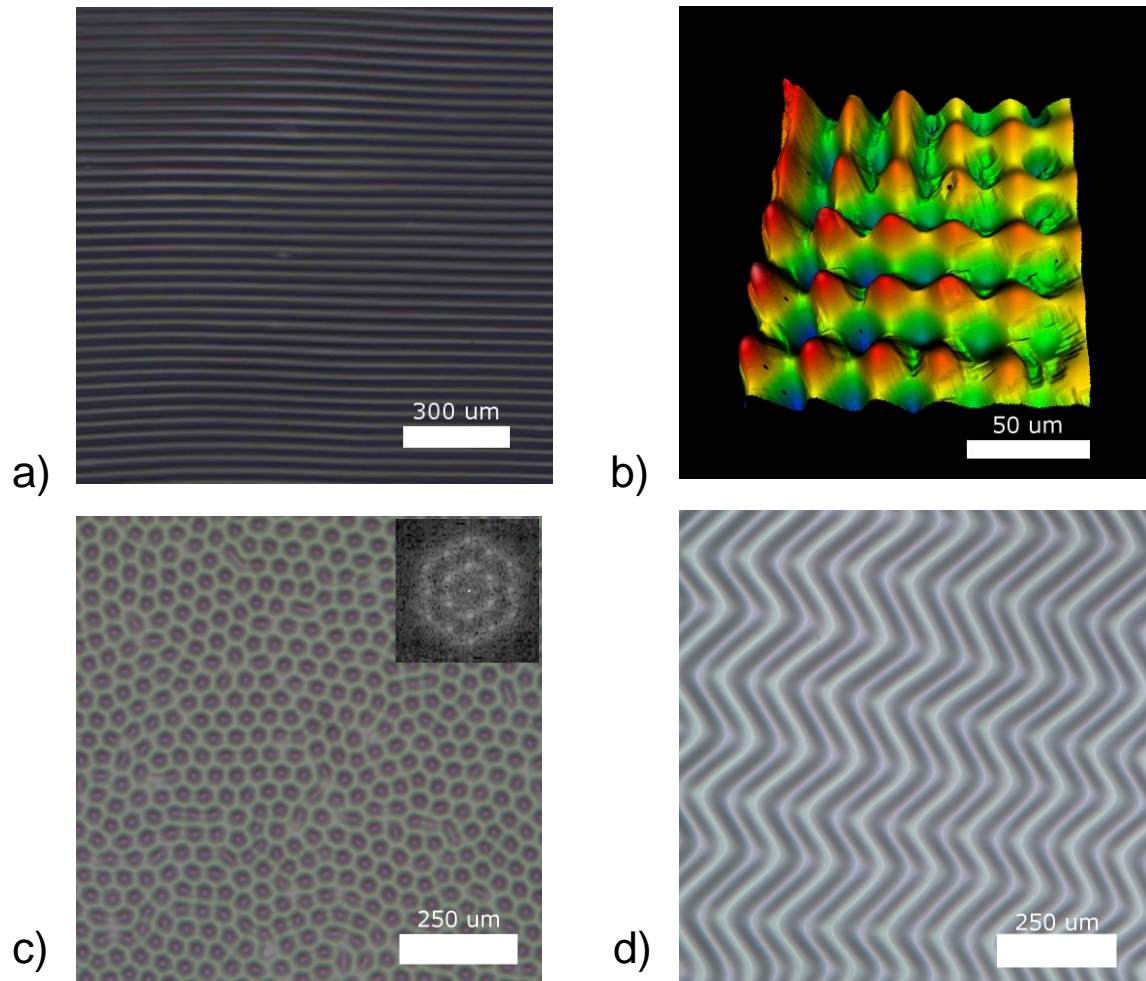
Fig. 2 Experimental observations of four buckling modes of films on PDMS substrates: a) 1D mode, observed when one principal in-plane stress dominates; b) square checkerboard mode; c) hexagonal mode (inset: fast Fourier transform of a selected "grain" of depressions, showing the hexagonal ordering); and d) herringbone mode. Images a , c , and d are optical micrographs of wrinkles generated via the swelling process outlined in Section 2. Image b depicts the surface profile of a flat polystyrene film on a PDMS substrate, wrinkled due to thermal mismatch stresses. The checkerboard pattern in image b is not readily observed. In this case it occurred within a relatively small region surrounded by other wrinkle patterns.
