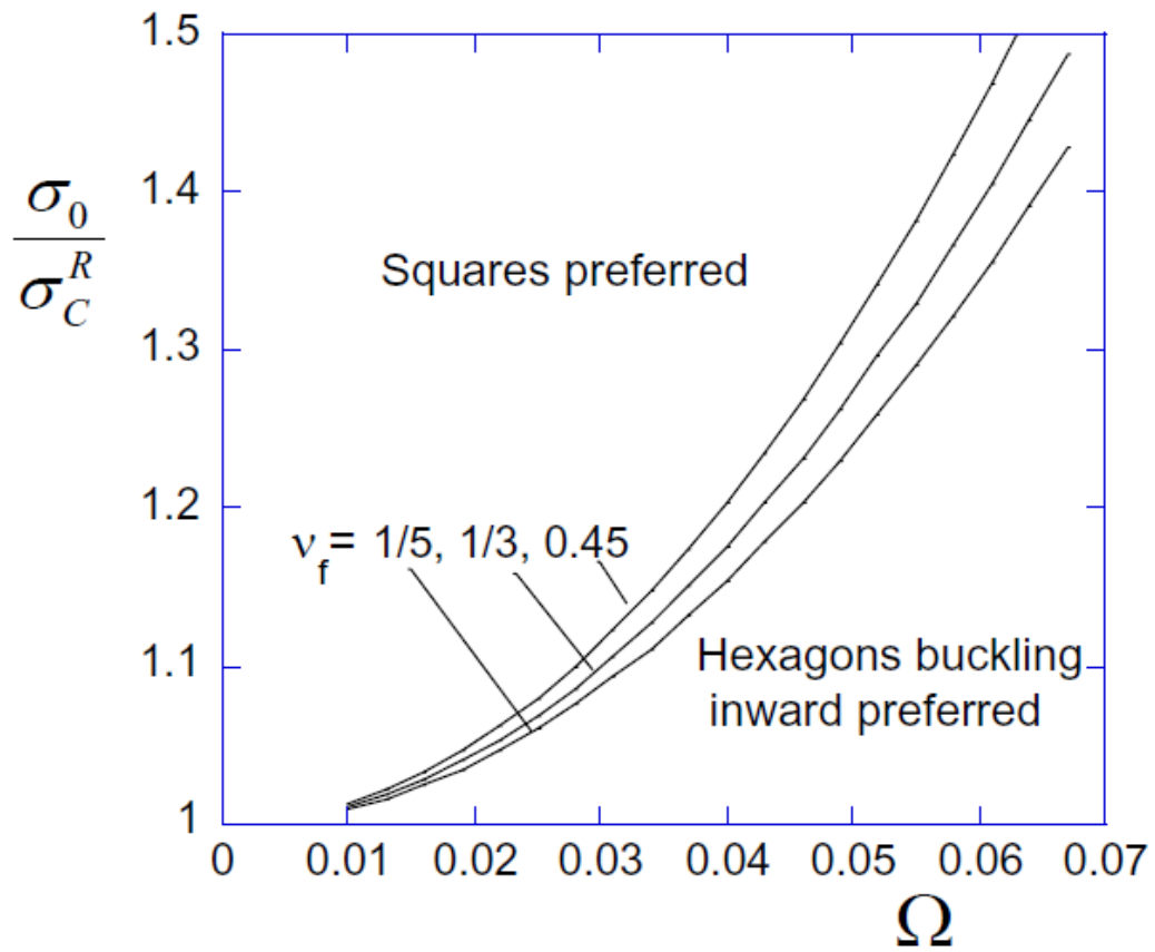
Fig. 13 For a given \nu_f the curve gives the value of \Omega for which the energy of the hexagonal mode (buckling inward) equals that of the square mode. A mode-selection criterion based on minimum energy favors the hexagonal mode to the right of the curve and the square mode to the left of the curve.
