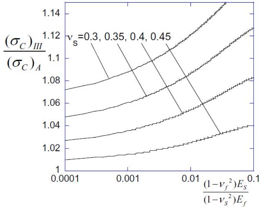
Fig. 6 The exact critical stress, (\sigma_C)_{III} for plane strain deformation of the film/substrate system for various Poisson ratios of the substrate with (\sigma_C)_A = (\bar{E}_f / 4)(3\bar{E}_s / \bar{E}_f)^{2/3} . The film layer is incompressible.
