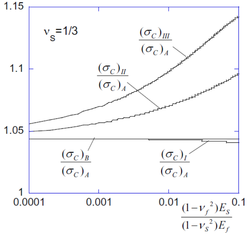
Fig. 5 Critical stress for plane strain deformation of the film/substrate system with \nu_s = 1/3 . The reference is (\sigma_c)_A = (\bar{E}_f / 4)(3\bar{E}_s / \bar{E}_f)^{2/3} ; (\sigma_c)_B = (\bar{E}_f / 4)(3\bar{E}_s^* / \bar{E}_f)^{2/3} with \bar{E}_s^* = 4(1 - \nu_s)^2 \bar{E}_s / (3 - 4\nu_s) . Cases (I), (II) and (III) are described in the text; (\sigma_c)_{III} is exact.
