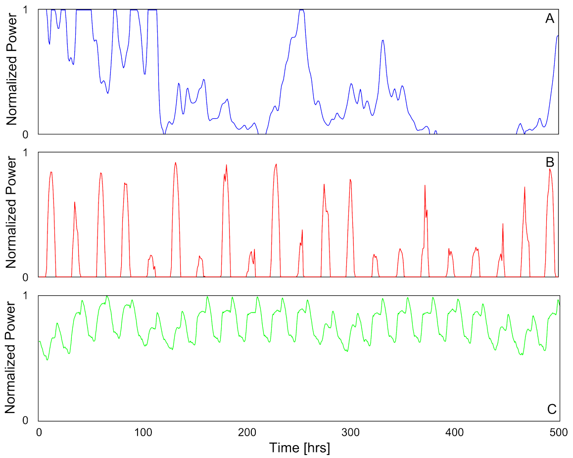
Figure 1: (A) The normalized shape of wind power calculated from real wind speed data in Wilhelminadorp, Netherlands, by applying the power curve for a GE 1.5MW turbine [3, 4, 5]. (B) The normalized shape of solar PV power output in January in Boston, MA, USA [6]. (C) The normalized shape of electricity demand in the UK from the National Grid website [7]. N.B. The data shown are a 500 hour subset of the larger range used for normalization.
