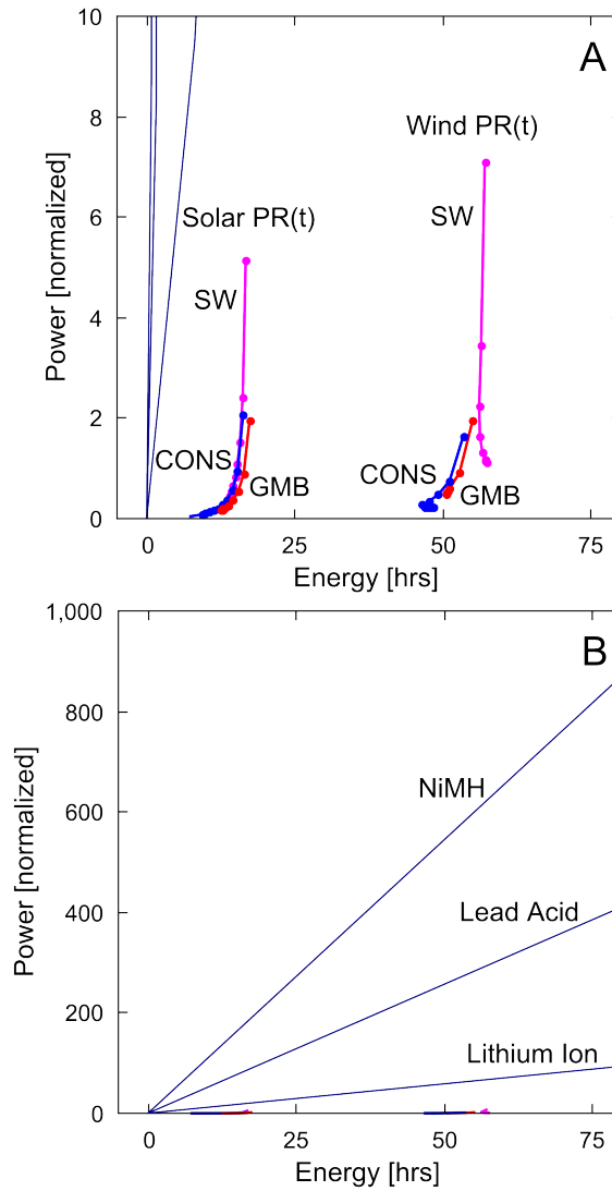
Figure 7: (A) Power and energy requirements, normalized to peak wind or PV production capacity, for several supply scenarios. All the results for the solar PV are grouped to the left below 25 hrs. All the results for wind are grouped to the right near 50 hrs. In different colors are the different SU(t) scenarios; SW in pink, GMB in red, and CONS in blue. The highest point on each line corresponds to 95% system efficiency, and the efficiency decreases in 5% increments with each successive point downwards. (B) The same exact data plotted with a vertical axis scale, showing the vast difference in power scales between common solid-electrode batteries and intermittent renewable electricity storage requirements. The same lines appear nearly vertical in (A) and are unlabeled.
