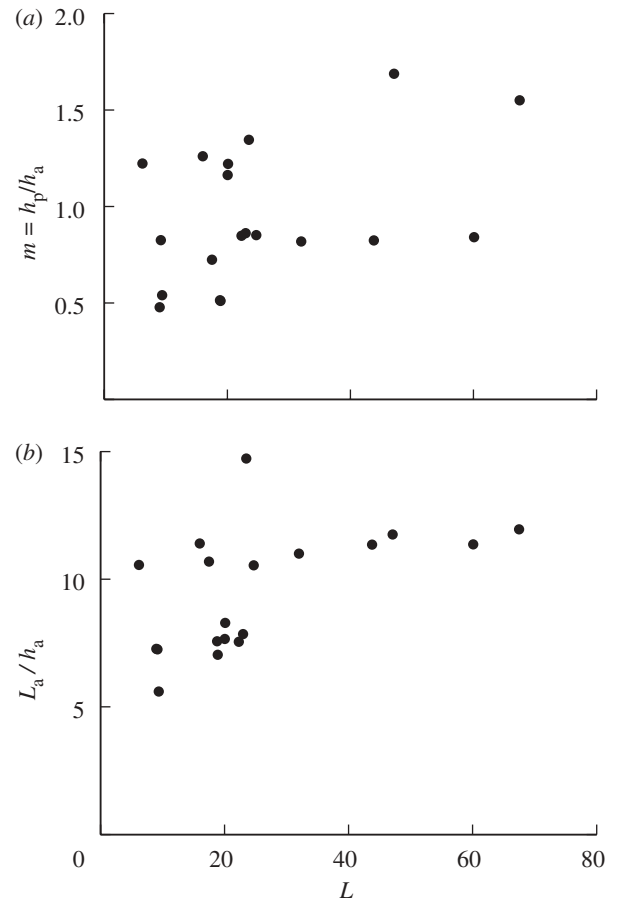
Figure 3. (a) Ratio m of thicknesses and (b) aspect ratio L_a/h_a as a function of the length L of scales from different pine cones. Although the data are strongly scattered, both m and L_a/h_a are found to be weakly dependent on the scale's size L .
