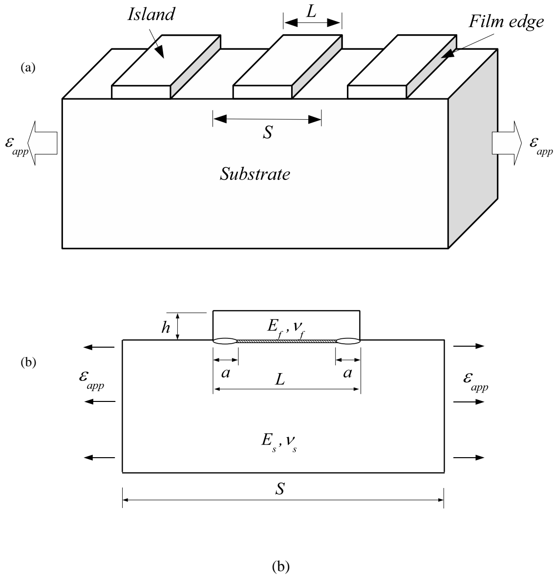
Fig. 1. (a) Schematics of a lattice of thin film functional islands on compliant substrate, which is subject to uniaxial tensile strain \epsilon_{app} . Subscript “f” denotes “film” and “s” means “substrate”. L is the island size and S is the island spacing. The thickness for film and substrate are h and H respectively. (b) Schematics of the plane strain model for one cell, where a is the crack size.
