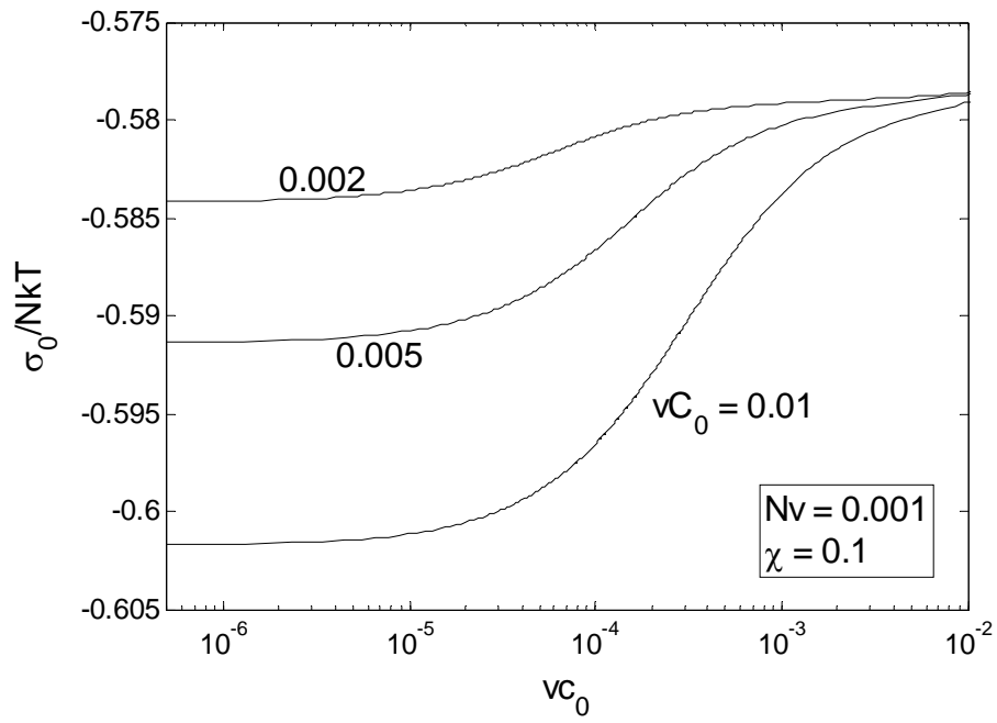
Figure 6. A blocking stress develops in a gel swelling under a constraint.
