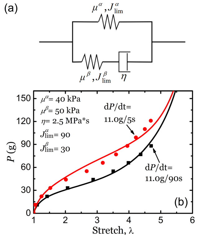
FIG. 3. (Color online) (a) Viscoelastic relaxation is modeled with a dashpot and two nonlinear springs. (b) With no voltage applied, the mechanical load vs stretch of the discs was measured at 2 loading rates of 11.0 g/5 s and 11.0 g/90 s. The symbols are experimental data, while the curves show the fitting with the viscoelastic model.
