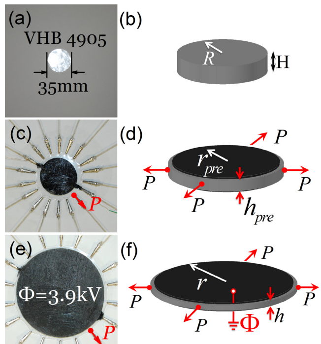
FIG. 1. (Color online) (a, b) Photograph and schematic of a circular disc of VHB, thickness H=0.5 mm and radius R=17.5 mm, before applying a voltage. (c) Attachment of loading weights (eighteen in number). (d) Under the dead load, the radius and thickness become r_{pre} and h_{pre} , respectively. Both surfaces of the disc are coated with electrodes of carbon grease. (e, f) When both the dead load and voltage, \Phi , are applied, the radius r increases and the thickness h decreases. The photos (a, c, e) are all taken at the same magnification. Comparison of (c) and (e) shows a voltage-actuated stretch of r/r_{pre}=2.4 in this particular example.
