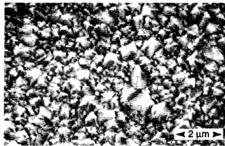
Fig. 1. Scanning electron micrograph revealing the microstructure of the diamond coating on the titanium alloy.
