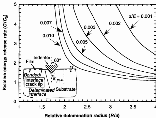
Fig. 3. Trends in the energy release rate with changes in the delamination radius and a schematic of the adhesion test with a diamond indenter (inset).
