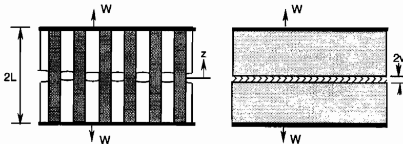
Fig. 2. Fiber bridging prototype and spring model; the average applied stress is \sigma .
