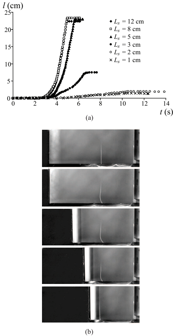
Fig. 5: (a) Retracted length of 53 \mu m thick tracing paper samples as a function of time. Narrow strips retract slowly due to the influence of the transverse curvature that predominates in the neighborhood of the edges. (b) 25 cm long and 15 cm wide strip of 65 \mu m thick tracing paper retracting on water, seen from above. The right end is held clamped while the left extremity is free to curl. The bright line is due to a laser sheet shining from right to left, almost parallel to the water surface. Initially straight when the sheet first contacts water, the line curves as water diffusion induces upward curling along the paper's edges. Before being taken up by the rolling cylinder, the paper flattens as revealed by the straightening of the laser line probe. The pictures were taken 2.6, 5.8, 7.5, 7.8 and 7.9 s after contact with water.
