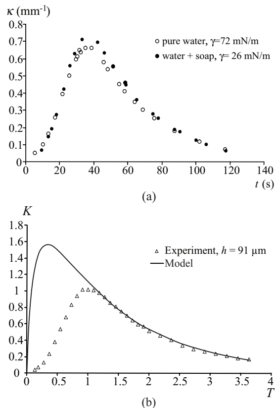
Fig. 3: (a) The bending dynamics of a 77 \mu\text{m} thick paper sample on pure water (surface tension \gamma = 72 \text{ mN/m} ) and on water with surfactants ( \gamma = 26 \text{ mN/m} ) is identical, showing that water is transported by molecular diffusion rather than capillary imbibition. (b) Rescaled curvature of a paper strip as a function of non-dimensional time as predicted by assuming a smooth diffusive front for the water content profile. At long times, the model fits experimental data very well, while the short-time behavior is due to the complex variation of the modulus as a function of the water volume fraction and the swelling of the paper normal to its plane.
